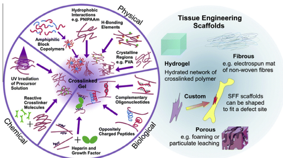
Fig. 10. Hydrogels in tissue engineering (reprinted from E.S. Place, J.H. George, C.K. Williams, M.M. Stevens, Chem. Soc. Rev. 2009, 38, 1139–1151 [123] with permission from the Royal Society of Chemistry).
