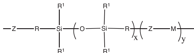
Fig. 5. General formula of the thermoplastic silicone-containing compositions employed by Lai et al. 'M' is a hydrophilic group; 'R' is an alkyl group with 1–10 carbon atoms that can be separated by ether, urethane or ureido linkages; 'R 1 ' is hydrogen, monovalent hydrocarbon groups or halogen substituted monovalent hydrocarbon moieties with 1–18 carbon atoms; 'Z' may be a divalent urethane or ureido portion; 'x' and 'y' are equal or greater than 1 [44].
