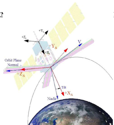
Figure 2: SMOS measurement observation mode geometry. Ref [5]
