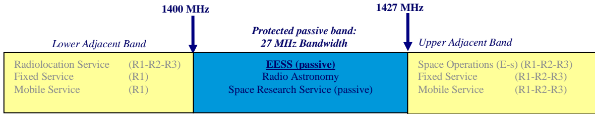
Figure 3: Schematic about frequency allocation to the EESS passive in the 1400-1427 MHz band
