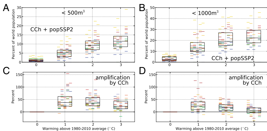
Fig. 3. Percentage of world population living in countries with annual mean BW availability ( Materials and Methods ) below 500\text{ m}^3 per capita ( Left ) and below 1,000\text{ m}^3 per capita ( Right ). Symbols as in Fig. 2. ( A and B ) RCP8.5 climate scenario, population change according to SSP2. ( C and D ) Amplification by climate change of the level of water scarcity that is expected from population change alone; computed as the difference between a constant-climate scenario ( SI Appendix, Fig. S7 ) and the full scenario shown above, divided by the constant-climate scenario, and expressed as percentage (so that the population-only case equals 100%). For example, in C , the MMM indicates that at 2\text{ }^\circ\text{C} global warming, climate change amplifies the level of absolute water scarcity (number of people below 500\text{ m}^3 per capita) expected from population change alone by about 36%.
