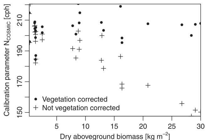
Figure 7. The COSMIC calibration parameter N_{\text{COSMIC}} without ( N_{\text{epithr}} \sigma = 20 cph) and with vegetation-corrected neutron intensity ( N_{\text{epithr}} \sigma = 9 cph).
