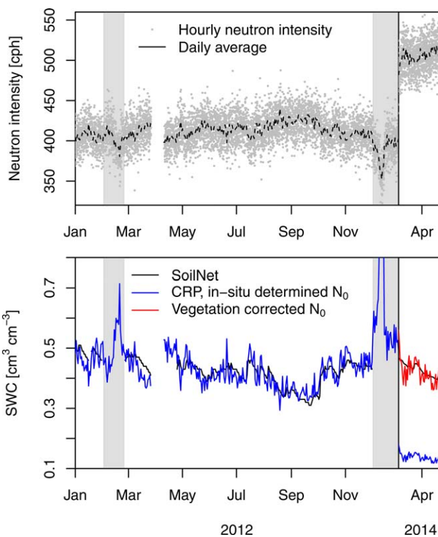
Figure 5. Measured corrected neutron intensity ( N_{epih} ) from the Wuestebach CRP, hourly (gray dots), and daily averaged (dashed). The lower figure shows daily volumetric soil water content estimated with the calibrated site-specific N_0 (blue) and with the N_0 estimated from the vegetation correction function (red) under deforested conditions. The black line represents horizontally and vertically weighted soil water content measured with SoilNet. Gray shaded areas indicate periods with snow.
