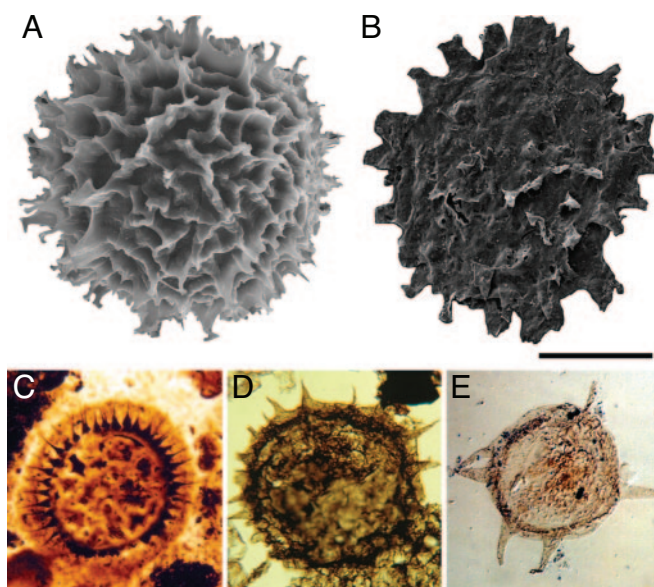
Fig. 3. Morphologies of LOEM taxa and a modern analog. (A) SEM of resting cyst, modern arthropod Brachinella longirostris . (B) Alicesphaeridium sp., Vychegda Formation, northern Russia. (C) LOEM microfossil, Doushantuo Formation, China. (D) LOEM microfossil, Officer Basin, Australia. (E) LOEM microfossil, Kursovsky Formation, Siberia. (Scale bar: 100 \mu\text{m} for A and D; 200 \mu\text{m} for B and C; 150 \mu\text{m} for D and E.)
