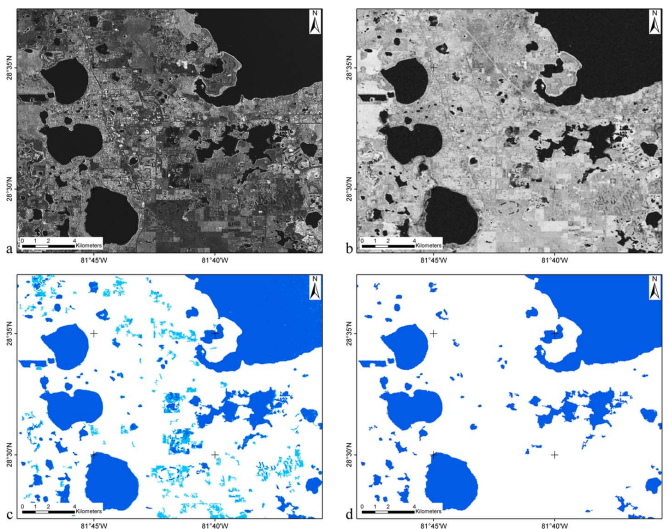
Fig. 4. (a) Amplitude image of the second study area around Lake Apopka in the west of Orlando, USA, acquired on 12th February 2011, (b) corresponding coherence image, (c) Water body detection mask derived from the amplitude image: first amplitude threshold detections displayed in dark blue, second's in light blue, (d) Water body detection mask derived from the coherence image.
