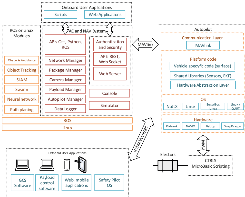
Fig. 18. Software architecture (acc. these authors)
