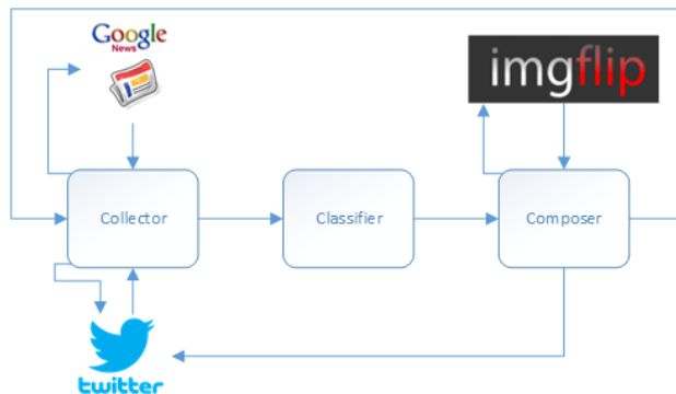
Figure 1: High-level architecture of MEMEGERA 2.0.
