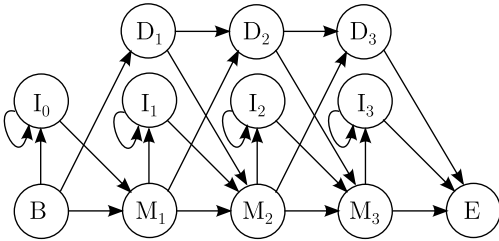
Fig. 5. Example of a profile HMM. States M_k are match states, I_k are insert states and D_k are delete states. States B, E , and D_1 \dots D_3 are silent, which means that they do not generate any characters.
