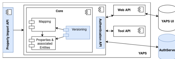
Figure 3: Architecture of the YAPS system. Components in blue remain future work.
