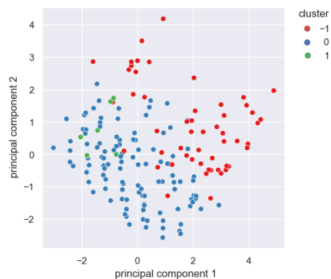
Figure 6: DBSCAN clustering
