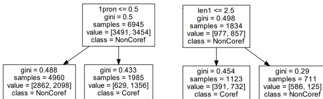
Figure 3: Subtree of the decision tree (3)
