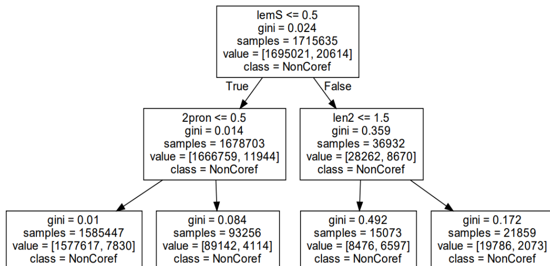
Figure 1: Subtree of the decision tree (1)
