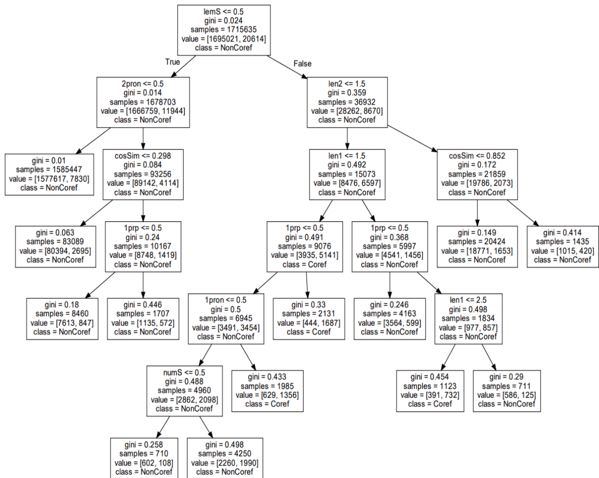
Figure 6: Decision tree
