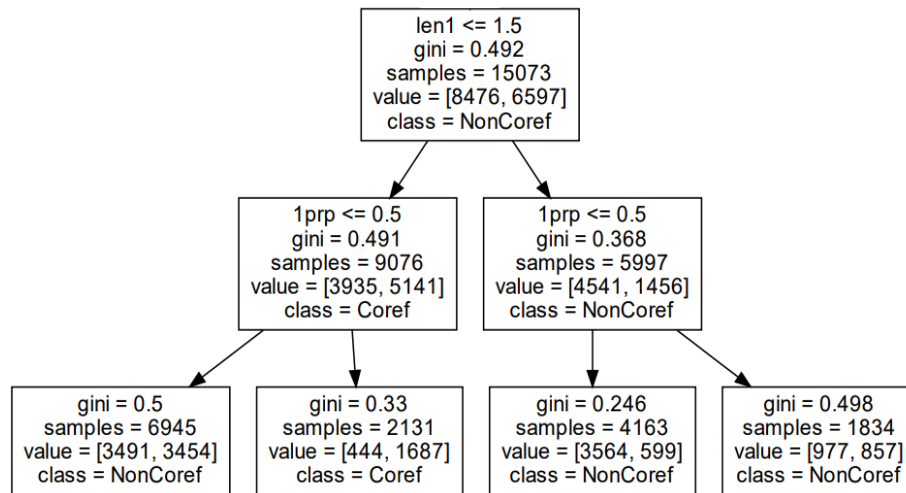
Figure 2: Subtree of the decision tree (2)
