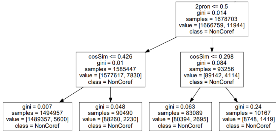
Figure 5: Subtree of the decision tree (5)
