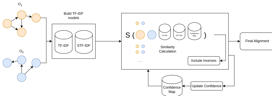
Figure 1: PropMatch architecture.
