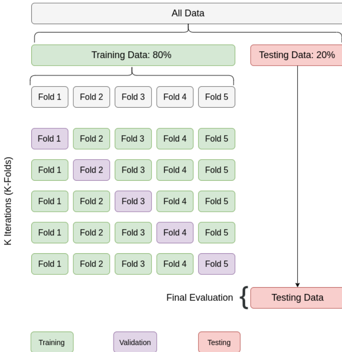
Fig. 4. K-Fold Validation
