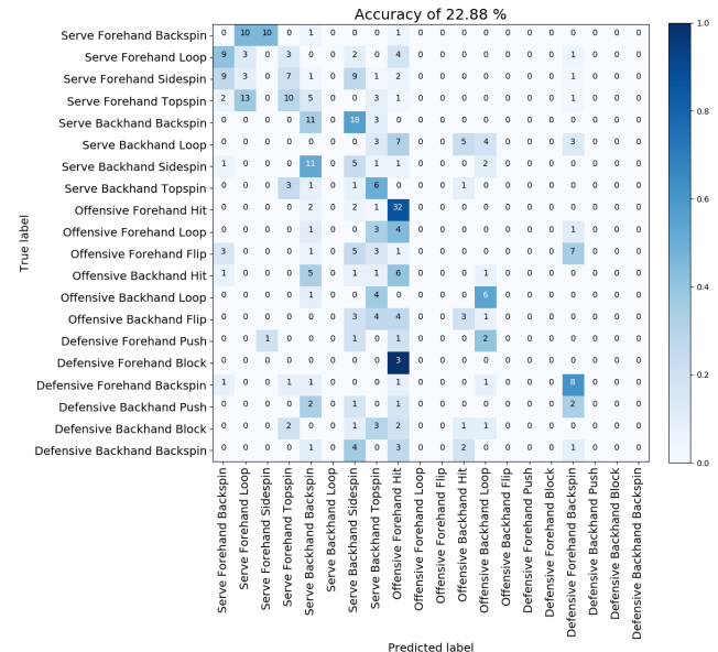
Figure 2: Confusion Matrix of our best run
