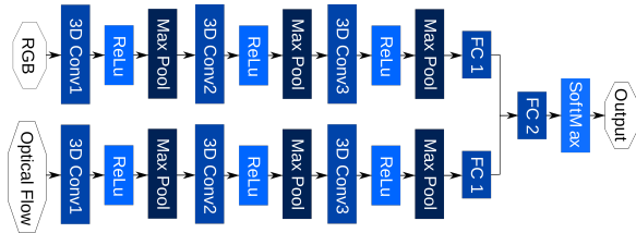
Figure 1: SSTCNN architecture
