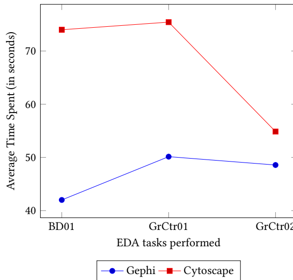
Figure 3: Temporal analysis efficiency for Cytoscape and Gephi
