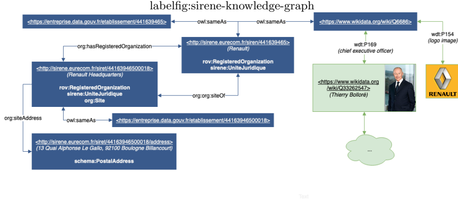
Fig. 1. An example of a legal unit and its establishment modeled using the Sirene ontology for the French company Renault
