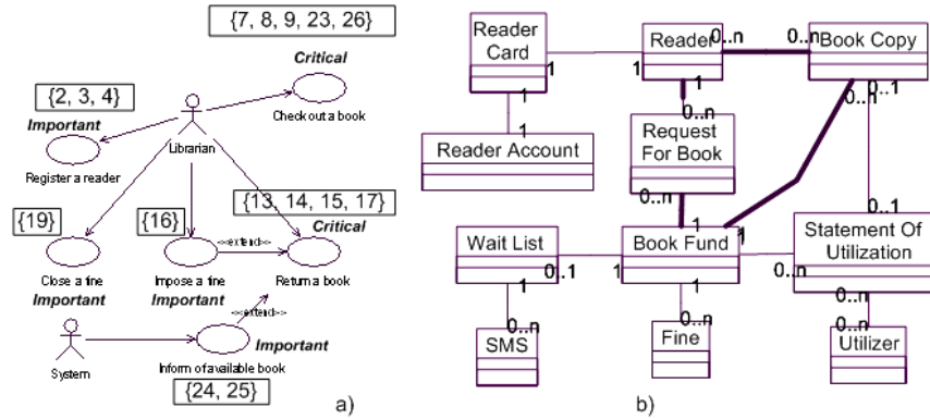
Fig. 4. The use case model (a); and the initial conceptual model (b)
