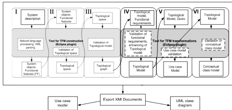
Fig. 5. The scheme of the tool supporting the TFMfMDA
