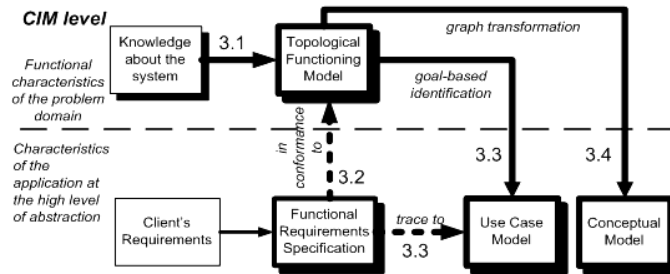
Fig. 2. CIM creation with the TFMfMDA in the OOA
