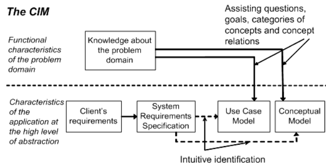
Fig. 1. The current state of CIM creation in the OOA
