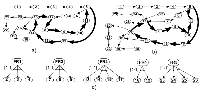
Fig. 3. Topological space of the library functioning (a), the modified topological space of the library functioning (b), and requirement mappings onto the functional features (c)
