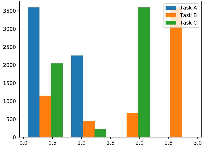
Fig. 1. Data distribution
