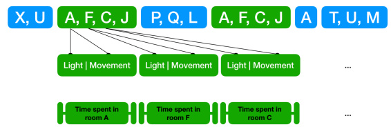
Figure 2: Identified patterns in an action sequence.
