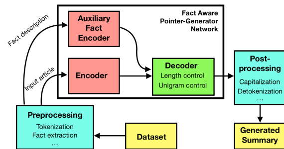
Figure 1: Fact aware pointer-generator network.
