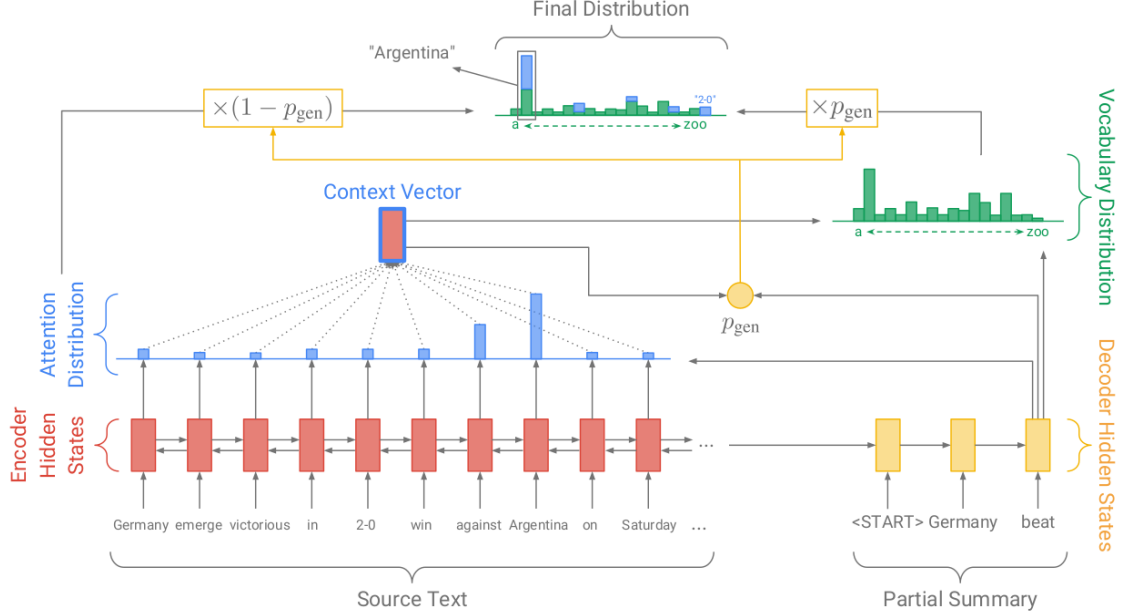
Figure 2: From (See et al., 2017). The source text gets encoded by a bidirectional LSTM and decoded by an unidirectional LSTM. At each decoding step t , an attention distribution a^t is computed. From a^t , we derive the pointer distribution P_{\text{pointer}} by summing up the probabilities of all occurrences per input token. To get the final distribution P from which tokens are generated, we add the vocabulary distribution P_{\text{vocab}} (weighted by p_{\text{gen}} ) and P_{\text{pointer}} (weighted by (1 - p_{\text{gen}}) ). In-article OOVs have probability 0 under P_{\text{vocab}} and tokens that do not occur in the article have probability 0 under P_{\text{pointer}} . However, the sum of the two distributions, P , might yield strictly positive probabilities for all tokens of the extended vocabulary. One advantage is that in-article OOVs can still be generated by copying tokens from the source text.
