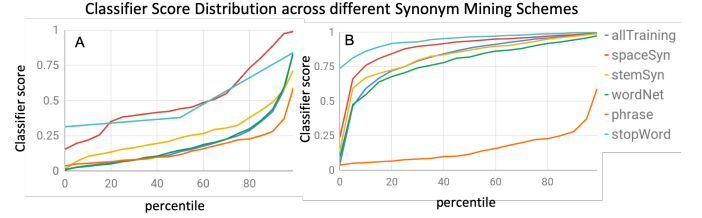
Figure 2: Classifier score distribution for A. negative class, and B. positive class
