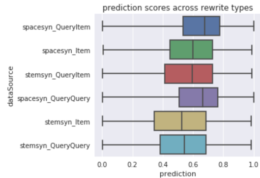
Figure 5: Prediction across different rewrite types
