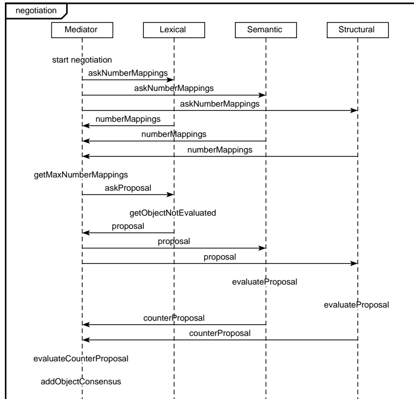
Figure 2: AUML negotiation interaction.
