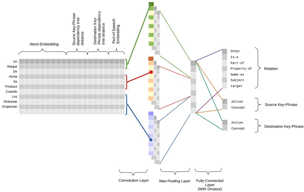
Figura 1: Layout of the proposed Convolutional Neural Network architecture
