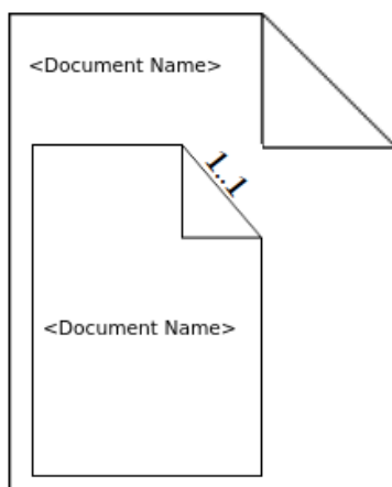
Figure 4: One-to-one relationship for embedded documents
