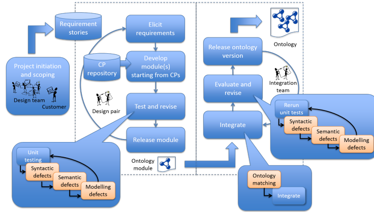
Fig. 1. Illustration of the integration of the detailed debugging and matching methods into XD. The rectangles represent activities already specified in the original version of XD (darker) and detailed activities that are proposed in this paper (lighter).
