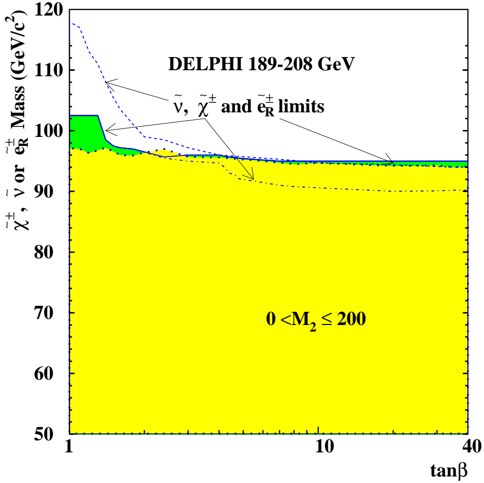
Figure 42: The minimum sneutrino mass (dark shading and the dashed curve) allowed by the slepton and neutralino searches, as a function of \tan\beta , together with the limits on the chargino mass (solid curve and dash-dotted curve), and the \tilde{e}_R mass (dotted curve and the light shading). The chargino mass limit indicated by the solid curve and the sneutrino and selectron mass limits were obtained assuming no mass splitting in the third sfermion family ( A_\tau - \mu \tan\beta = 0 in particular). The selectron mass limit is valid for M_{\tilde{e}_R} - M_{\tilde{\chi}_1^0} > 10 \text{ GeV}/c^2 . The chargino mass limit indicated with the dash-dotted curve was obtained allowing for mass splitting in the third sfermion family, with A_\tau = A_b = A_t = 0 .
