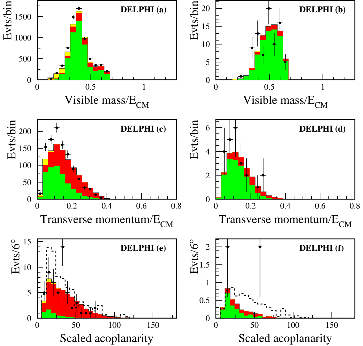
Figure 12: Comparison of real data from 2000 ( \sqrt{s} in the range 204–208 GeV) and simulation for the neutralino multijet selection without photons (a,c,e) and with photons (b,d,f), at the preselection (a,b),intermediate (c,d), and final selection(e,f) stages. The expected background (filled histogram) is divided into four-fermion (dark shading), two-fermion (intermediate shading), and two-photon processes (light shading). The distributions expected for \tilde{\chi}_3^0\tilde{\chi}_2^0 production with \tilde{\chi}_3^0 \rightarrow \tilde{\chi}_2^0q\bar{q} and \tilde{\chi}_2^0 decaying to \tilde{\chi}_1^0q\bar{q} or \tilde{\chi}_1^0\gamma are shown as dashed histograms where M_{\tilde{\chi}_3^0}=112 GeV/ c^2 , M_{\tilde{\chi}_2^0}=75 GeV/ c^2 and M_{\tilde{\chi}_1^0}=41 GeV/ c^2 . The signals are normalised cross-sections of 0.8 pb(e) and 0.2 pb(f).
