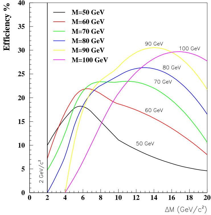
Figure 22: Signal efficiency of the stop search in the nearly degenerate scenario for different mass hypothesis as a function of \Delta M = M_{\tilde{t}_1} - M_{\tilde{\chi}_1^0} , for \sqrt{s}=189 and 206 GeV.
