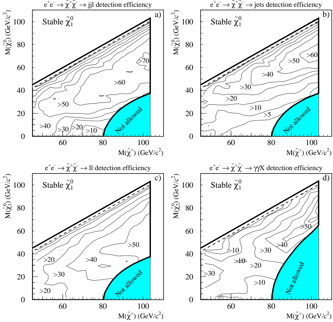
Figure 27: Chargino pair production detection efficiencies (%) for the four decay channels a) jj\ell , b) \text{jets} , c) \ell\ell and d) \text{rad} , at 206.5 GeV in the (M_{\tilde{\chi}_\pm}, M_{\tilde{\chi}_0}) plane. TPC sector 6 off and a stable \tilde{\chi}_1^0 are assumed. The shaded areas are disallowed in the MSSM scheme.
