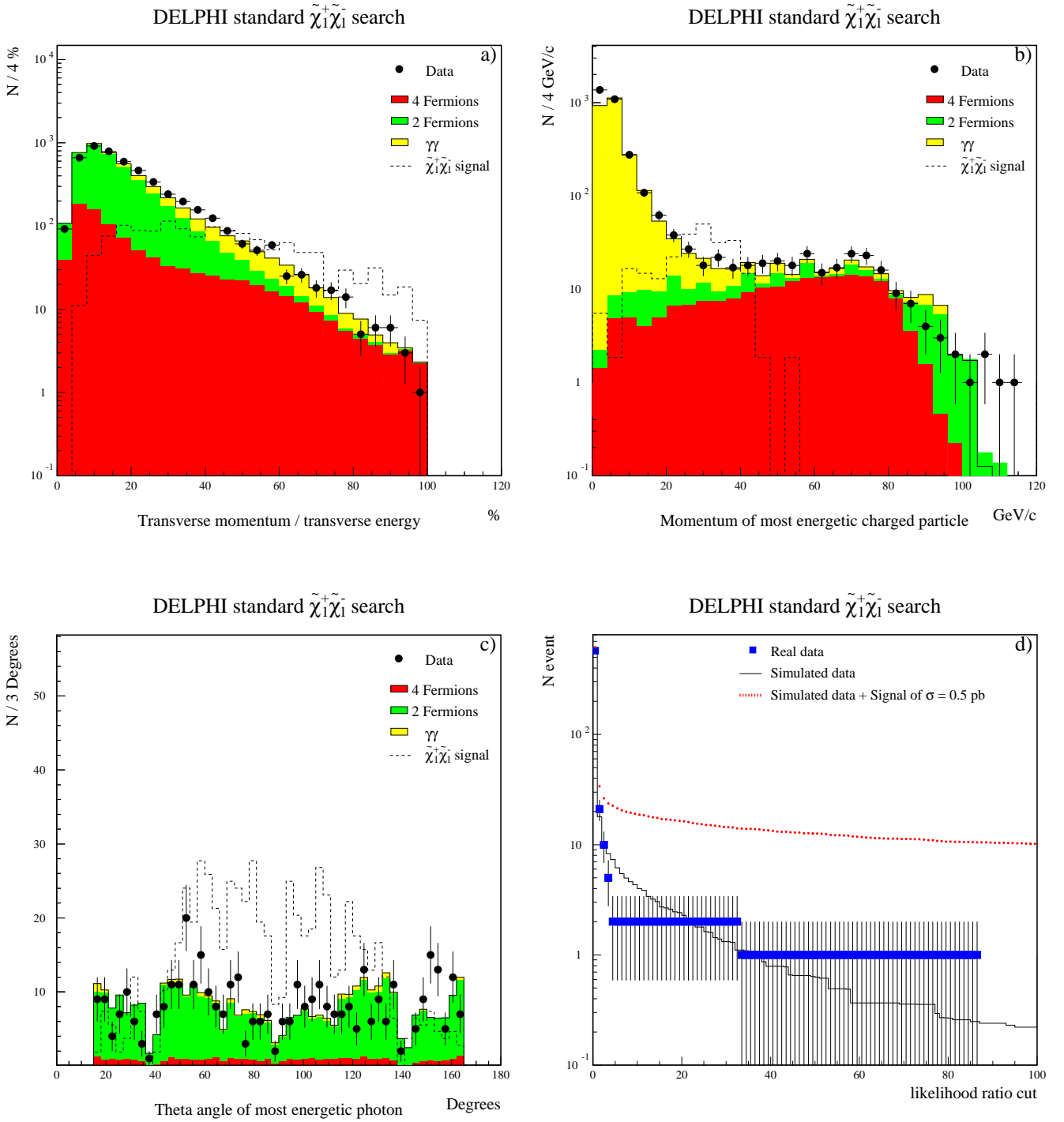
Figure 7: a), b) and c) show comparisons between real data (dots) and simulated background events (histogram) for the jets , \ell\ell and rad topologies respectively, using a logical OR of the 6 preselection cut functions of the corresponding topology. The hatched areas indicates how a characteristic chargino signal would appear. d) shows the number of events selected by the non-degenerate chargino analysis as a function of the \mathcal{L}_{RCUT} cut in the jjl topology for 25 \leq \Delta M < 35 GeV/ c^2 . The squares are the data and the solid line is the background simulation. The dotted curve shows a possible signal, M_{\tilde{\chi}_1^\pm} = 102.8 GeV/ c^2 , M_{\tilde{\chi}_1^0} = 73 GeV/ c^2 , of 0.5 pb added to the background. In all cases the data collected in the year 2000 with the TPC sector 6 on are shown.
