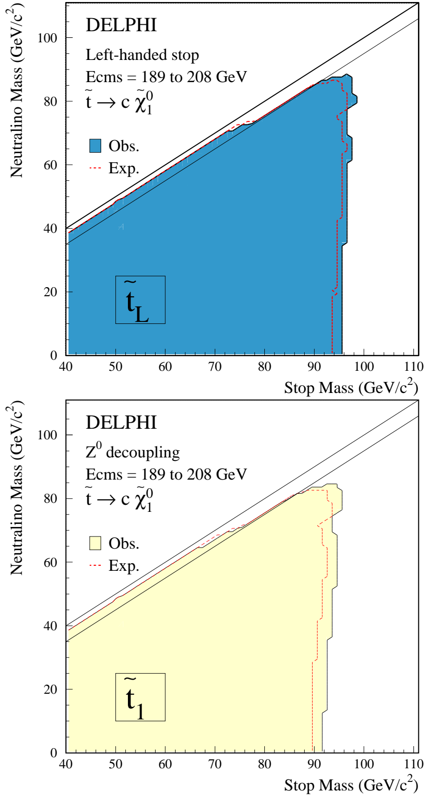
Figure 23: Excluded regions at 95 % confidence level for the stop search in the plane (M_{\tilde{t}_L}, M_{\tilde{\chi}_1^0}) for purely left handed stops (top) and for the states at the Z decoupling (bottom). The shaded region shows the observed excluded region and the line corresponds to the expected exclusion (for a discussion on the low stop mass region see section 6.3).
