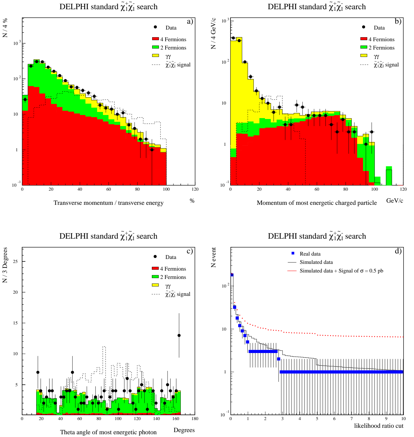
Figure 8: a), b) and c) show comparisons between real data (dots) and simulated background events (histogram) for the jets , \ell\ell and rad topologies respectively, using a logical OR of the 6 preselection cut functions of the corresponding topology. The hatched areas indicates how a characteristic chargino signal would appear. d) shows the number of events selected by the non-degenerate chargino analysis as a function of the \mathcal{L}_{RCUT} cut in the jj\ell topology for 25 \leq \Delta M < 35 GeV/ c^2 . The squares are the data and the solid line is the background simulation. The dotted curve shows a possible signal, M_{\tilde{\chi}_1^\pm} = 102.8 GeV/ c^2 M_{\tilde{\chi}_1^0} = 73 GeV/ c^2 , of 0.5 pb added to the background. In all cases the data collected in the year 2000 with the TPC sector 6 off are shown.
