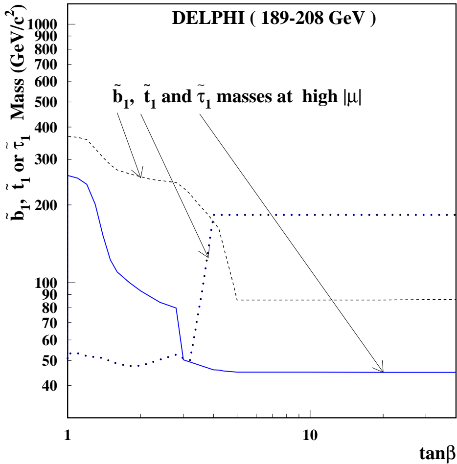
Figure 41: The masses as a function of \tan\beta of the lightest stau (solid curve), stop (dotted curve) and sbottom (dashed curve), at the highest allowed |\mu| for the lowest non-excluded M_2 value. Mass splitting in the stau (sbottom, stop) sector in the form A_\tau - \mu\tan\beta ( A_b - \mu\tan\beta , A_t - \mu/\tan\beta ) was assumed, with A_\tau = 0 ( A_b = A_t = 0 ).
