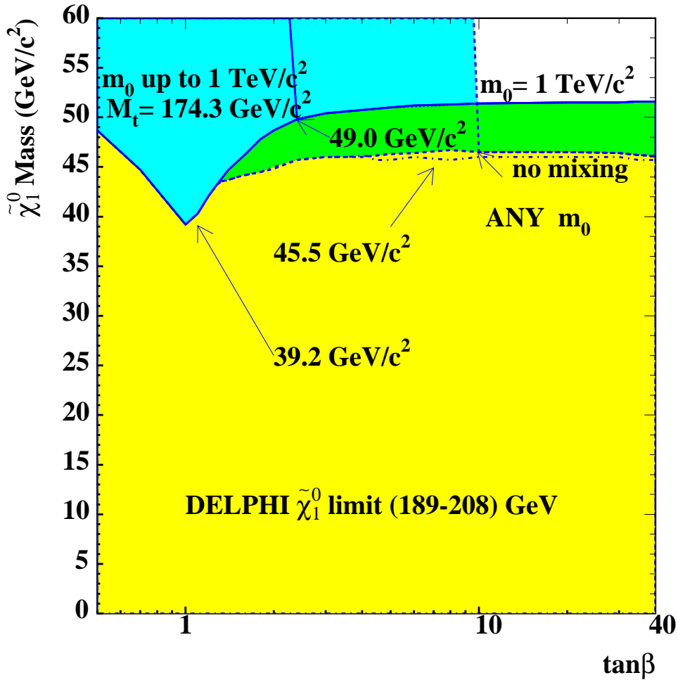
Figure 40: The lower limit at 95 % confidence level on the mass of the lightest neutralino, \tilde{\chi}_1^0 , as a function of \tan\beta assuming a stable \tilde{\chi}_1^0 . The solid curve shows the limit obtained for m_0 = 1000 \text{ GeV}/c^2 , the dashed curve shows the limit obtained allowing for any m_0 assuming that there is no mixing in the third family ( A_\tau = \mu \tan\beta , A_b = \mu \tan\beta , A_t = \mu/\tan\beta ), and the dash-dotted curve shows the limit obtained for any m_0 allowing for the mixing with A_\tau = A_b = A_t = 0 . The steep solid (dashed) curve shows the effect of the searches for the Higgs boson for the maximal M_{H^0} scenario (no mixing scenario), m_0 \leq 1000 \text{ GeV}/c^2 and M_t = 174.3 \text{ GeV}/c^2 , which amounts to excluding the region of \tan\beta < 2.36(9.7)
