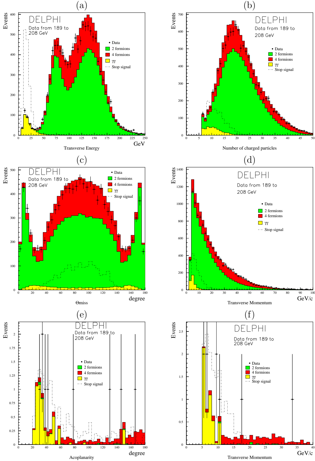
Figure 6: Comparison of data and simulation in the nearly degenerate squark analysis at preselection and final selection level. The distributions of the total transverse energy (a), total number of charged particles (b), angle between the missing momentum and the beam axis (c) and transverse momentum (d) are shown at preselection level. At the final selection level the acoplanarity (e) and transverse momentum (f) distributions are shown. All DELPHI data from 189 to 208 GeV is included. A signal corresponding to M_{\tilde{b}} = 60 \text{ GeV}/c^2 and \Delta M = 4 \text{ GeV}/c^2 is also shown, with arbitrary normalisation.
