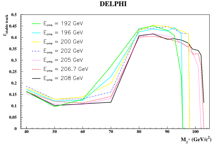
Figure 32: Efficiency for selecting a single almost stable chargino, as function of its mass, at the reference centre-of-mass energies collected by DELPHI in the years 1999 and 2000.
