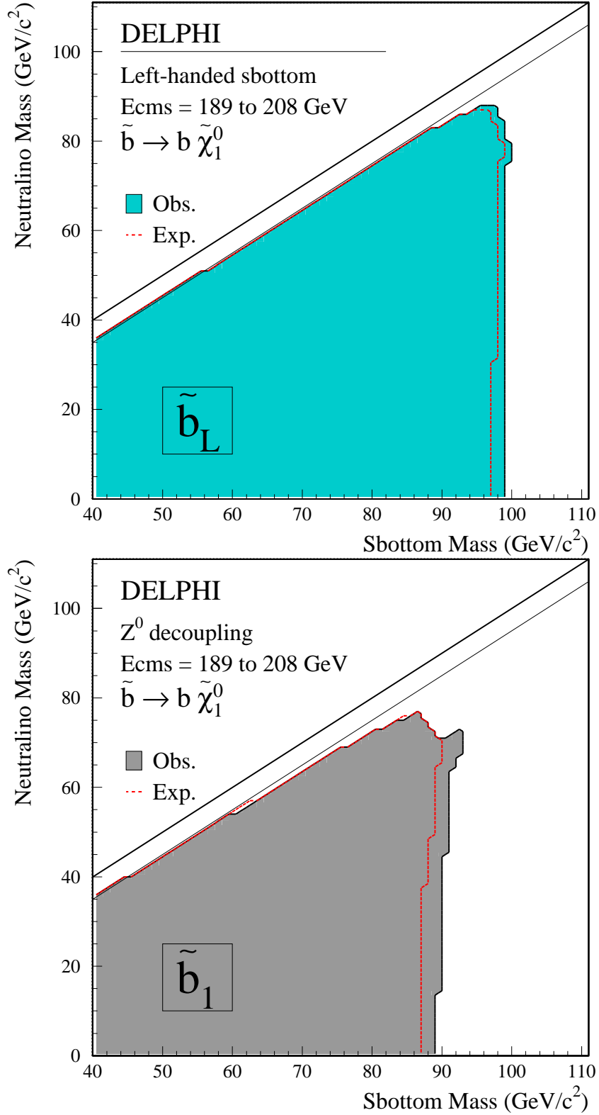
Figure 24: Excluded regions at 95 % confidence level for the sbottom search in the plane (M_{\tilde{b}_1}, M_{\tilde{\chi}_1^0}) for purely left handed sbottoms (top) and for the states at the Z decoupling (bottom). The shaded region shows the observed excluded region and the line corresponds to the expected exclusion (for a discussion on the low sbottom mass region see section 6.3).
