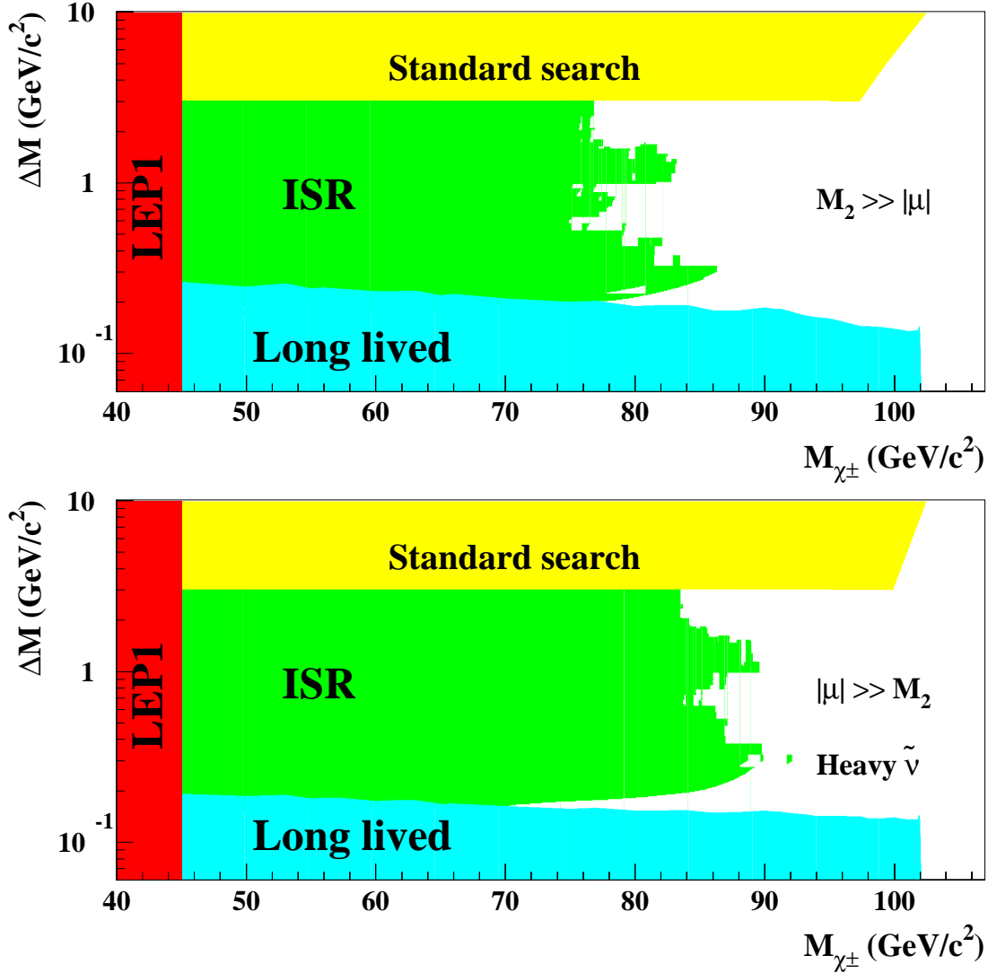
Figure 36: Regions in the plane (M_{\tilde{\chi}_1^+}, \Delta M) excluded by DELPHI at the 95% CL using: the search for high \Delta M charginos; the search for soft particles accompanied by ISR; and the search for long-lived charginos. The two scenarios are (a) the one in which the lightest chargino is a higgsino and (b) the one in which the lightest chargino is a gaugino. For the second scenario, the limits are valid in the heavy sfermion approximation, while for the higgsino scenario it is sufficient that M_{\tilde{f}} > M_{\tilde{\chi}_1^+} .
