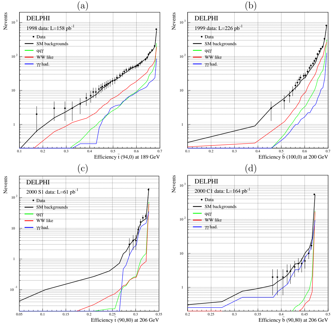
Figure 5: Number of events as a function of the signal detection efficiencies in the non-degenerate squark analysis: (a) 1998 data at 189 GeV: stop analysis for \Delta M > 20 \text{ GeV}/c^2 , (b) 1999 data from 192 to 202 GeV: sbottom analysis for \Delta M > 20 \text{ GeV}/c^2 , (c) 2000 data with TPC sector 6 off: stop analysis for 5 \leq \Delta M \leq 20 \text{ GeV}/c^2 , (d) 2000 data with TPC sector 6 on: sbottom analysis for 5 \leq \Delta M \leq 20 \text{ GeV}/c^2 .
