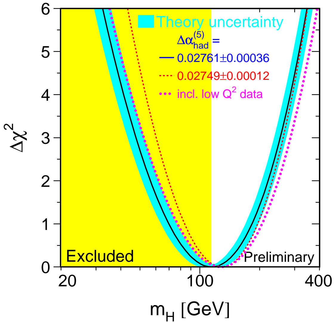
Figure 16.5: \Delta\chi^2 = \chi^2 - \chi_{min}^2 vs. m_H curve. The line is the result of the fit using all data (last column of Table 16.3); the band represents an estimate of the theoretical error due to missing higher order corrections. The vertical band shows the 95% CL exclusion limit on m_H from the direct search. The dashed curve is the result obtained using the evaluation of \Delta\alpha_{\text{had}}^{(5)}(m_Z^2) from Reference 299.
