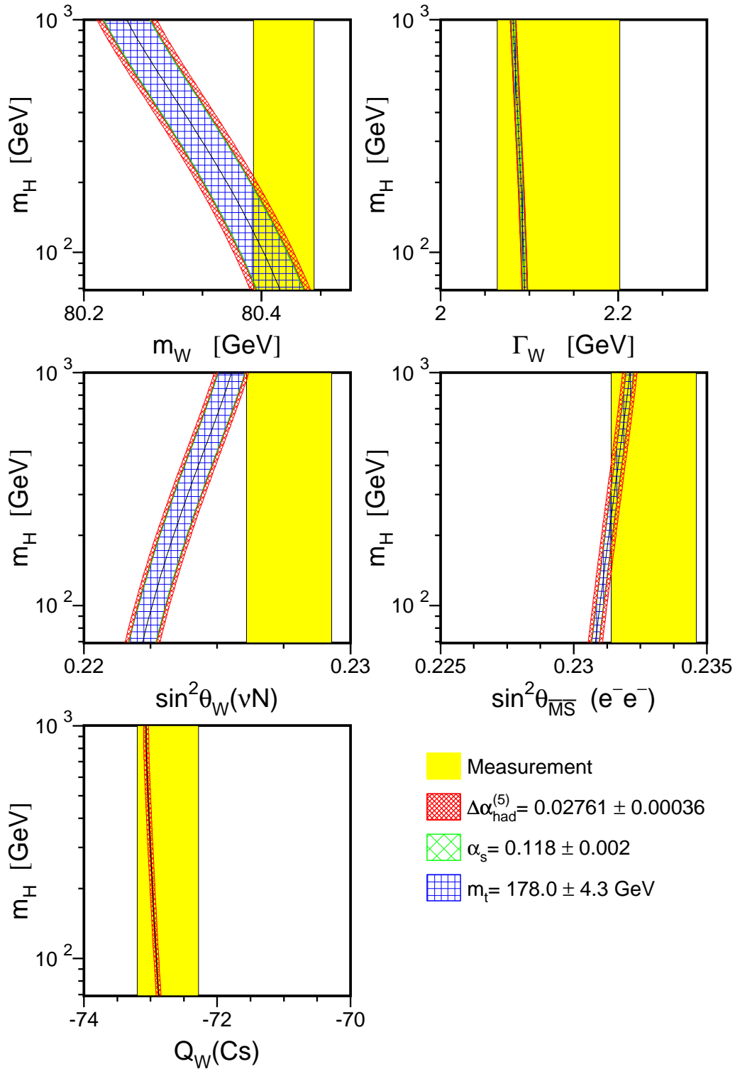
Figure 16.9: Comparison of m_W and \Gamma_W measured at LEP-2 and p\bar{p} colliders, of \sin^2 \theta_W measured by NuTeV and of APV in caesium with the Standard Model prediction as a function of m_H . The measurement with its error is shown as the vertical band. The width of the Standard Model band is due to the uncertainties in \Delta\alpha_{\text{had}}^{(5)}(m_Z^2) , \alpha_S(m_Z^2) and m_t . The total width of the band is the linear sum of these effects.
