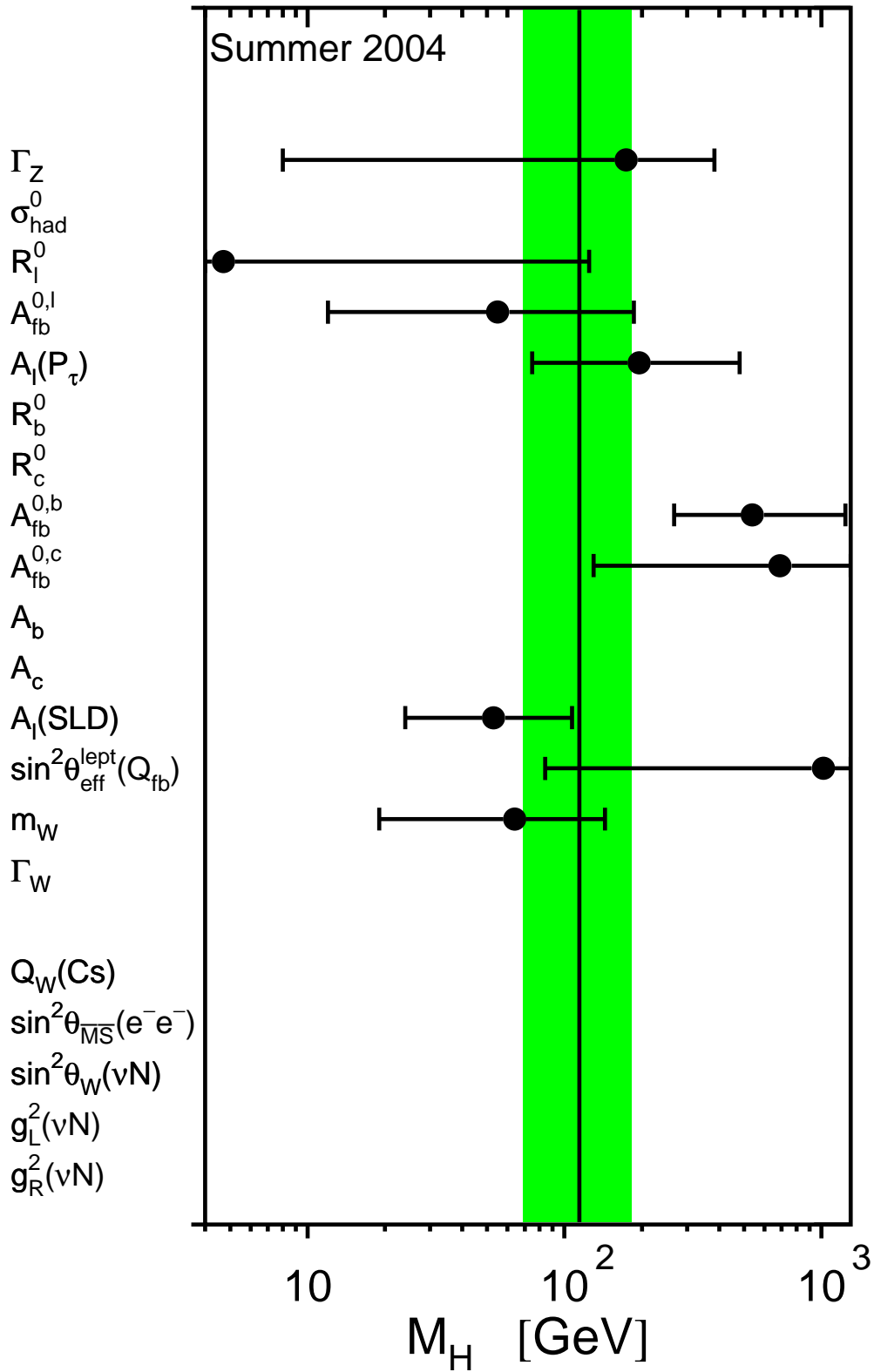
Figure 16.10: Constraints on the mass of the Higgs boson from each pseudo-observable. The Higgs-boson mass and its 68% CL uncertainty is obtained from a five-parameter Standard Model fit to the observable, constraining \Delta\alpha_{\text{had}}^{(5)}(m_Z^2) = 0.02761 \pm 0.00036 , \alpha_S(m_Z^2) = 0.118 \pm 0.002 , m_Z = 91.1875 \pm 0.0021 GeV and m_t = 178.0 \pm 4.3 GeV. Because of these four common constraints the resulting Higgs-boson mass values cannot be combined. The shaded band denotes the overall constraint on the mass of the Higgs boson derived from all pseudo-observables including the above four Standard Model parameters as reported in the last column of Table 16.3.
