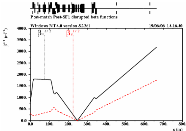
Figure 1: The matched linear optics for the 500 GeV extraction line, using the optimised NbTi final doublet layout.
