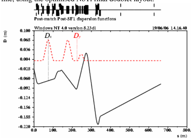
Figure 2: The matched dispersion functions for the 500 GeV extraction line, using the optimised NbTi final doublet layout.
