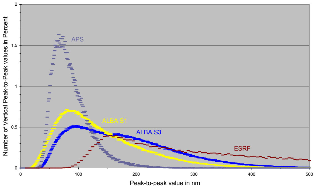
Figure 17: Relative number of vertical displacement peak-to-peak values at ALBA and two synchrotron light sources.
