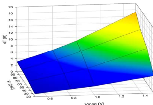
Figure 6: 3D plot of the dielectric heating \Delta T vs. modulation voltage amplitude and frequency.
