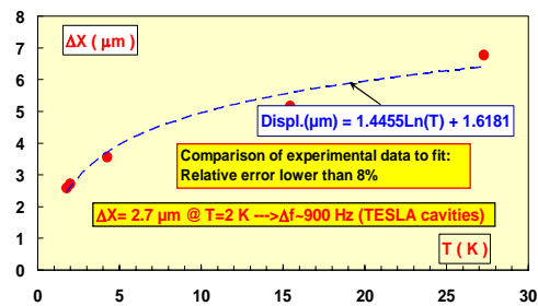
Figure 7: Variations of the full range ( V_{\text{max}}=120 V) displacement with temperature (Actuator: NOLIAC#1).
