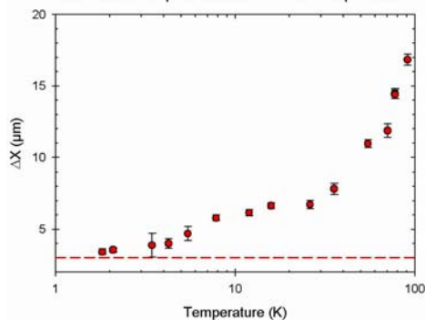
Figure 5: Variations of the full range ( V_{\text{max}}=120 V) displacement with temperature (Actuator: PICMA#1).
