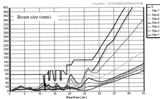
Figure 6: Beam size radii along the HEBT, with element errors ( 10^{-1} corresponds to 90% of the beam, 10^{-2} ? 99%, 10^{-3} ? 99.9%, and the black one: 100%).
