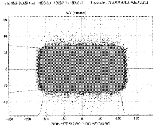
Figure 3: Output HEBT beam distribution at the target.
