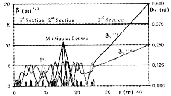
Figure 1: HEBT line optical functions.
