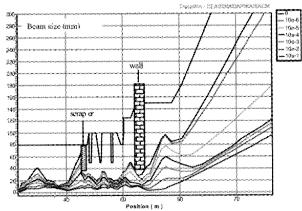
Figure 4: Beam size radii along the HEBT, without element errors ( 10^{-1} corresponds to 90% of the beam, 10^{-2} ? 99%, 10^{-3} ? 99.9%, and the black one: 100%).
