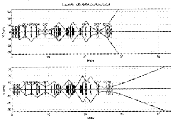
Figure 2: Transverse beam envelopes.
