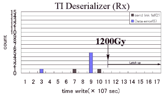
Figure 5: Time dependence of error incidence versus proton irradiation time for deserializer (Rx) chips of NS and TI. TI one was broken after 1200Gy irradiation.
