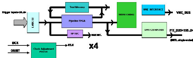
Figure 4: Block diagram of the CTP_IN module
