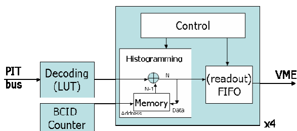
Figure 7: Block diagram of the CTP_MON module
