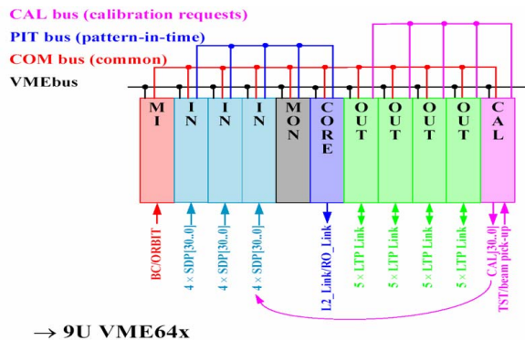
Figure 2: CTP design with its modules, backplanes, and signals
