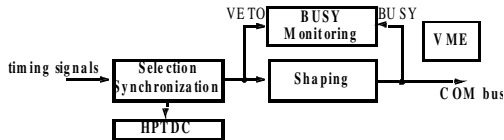
Figure 3: Block diagram of the CTP_MI module
