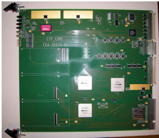
Figure 6: Photograph of the CTP_CORE module
