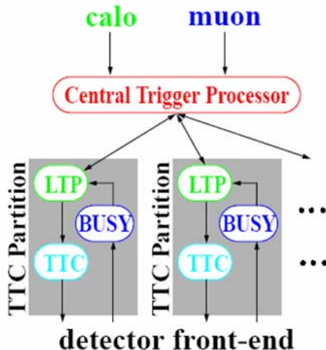
Figure 1: Overview of the ATLAS level-1 trigger The central trigger system consists of the CTP and the TTC partitions.
