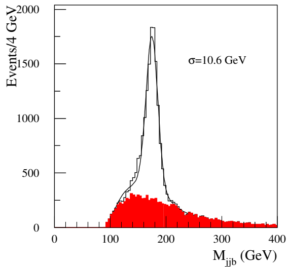
Fig. 1. Invariant mass of the bjj system after 10 \text{ fb}^{-1} of integrated luminosity. The shaded area is the combinatorial background
