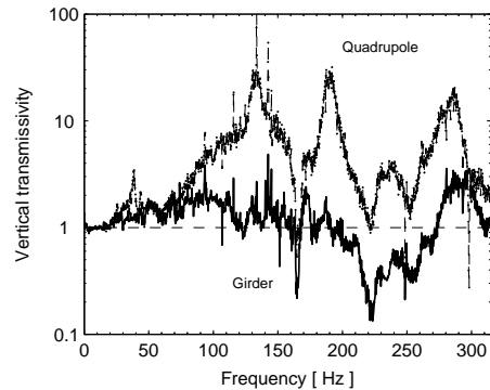
Figure 5: Vertical transmission from ground to girder (solid line) and to quadrupole (dotted).
