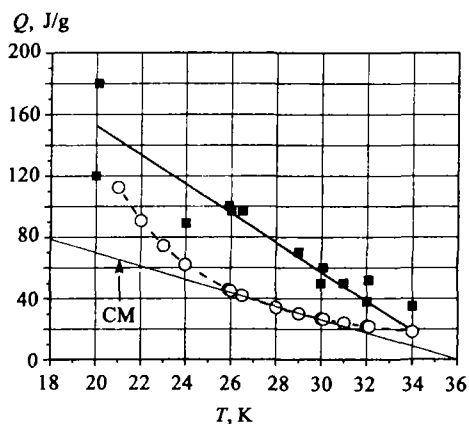
Fig. 3. Chemical stored energy in solid methane Q versus temperature of methane T . Black squares — amount of stored energy in induced burps versus temperature of ignition; open circles — saturated quantity of stored energy versus irradiation temperature; line CM — amount of stored energy in spontaneous burps of IPNS moderators [3], linear approximation of the authors
