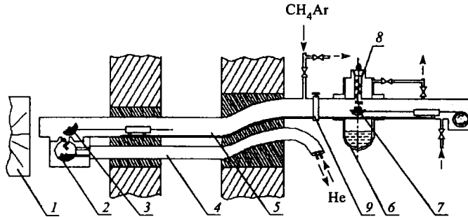
Fig. 1. Sketch of the URAM-2 cryogenic irradiation facility: 1 — the IBR-2 reactor; 2 — irradiation capsule; 3 — carrying bowl with a cart in «near the reactor» position; 4 — helium pipelines; 5 — evacuated transport passage; 6 — nitrogen cryostat; 7 — carrying bowl with a cart in «out of the reactor» position; 8 — charging tube with a plug; 9 — vacuum lock
