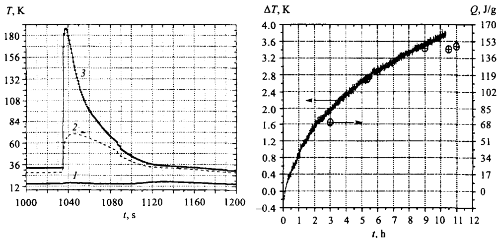
Fig. 4. Spontaneous release of stored energy in water ice: temperature excursion versus time. 1 — temperature of cooling helium; 2 — temperature of copper walls of the irradiation capsule; 3 — temperature of methane at 8 mm off the walls
