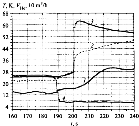
Fig. 2. Induced, fast release of stored energy in solid methane: temperature excursion versus time. 1 — temperature of cooling helium; 2 — temperature of copper walls of the irradiation capsule; 3 — temperature of methane at 8 mm off the walls; 4 — helium flow rate, 10 \text{ m}^3/\text{h}
