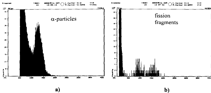
Figure 3. Ionization chamber spectra measured in the He/Ar/methane (45:45:10) mixture:
