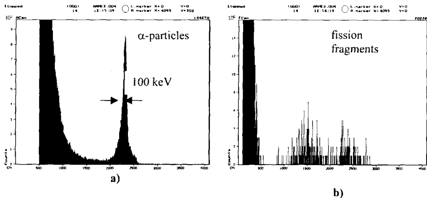
Figure 2. Ionization chamber spectra measured in the Ar/methane (90:10) mixture:
