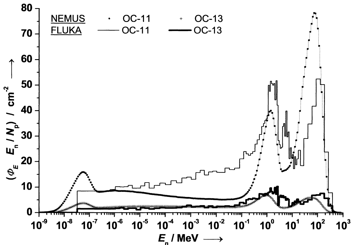
FIG 4 Absolute comparison of measured (NEMUS) and calculated (FLUKA) neutron spectra at two positions outside the cave for ^{12}\text{C} ions with 400 MeV/u impinging on a thick graphite target The spectra are presented in a lethargy plot per N_p = 10^{10} ions
