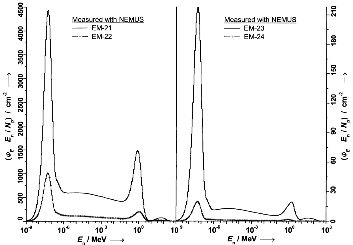
FIG 3 Measured neutron spectra, unfolded with MAXED, in the entry maze for ^{12}\text{C} ions with 400 MeV/u impinging on a thick graphite target. The spectra are presented in a lethargy plot per N_p = 10^{10} ions.
