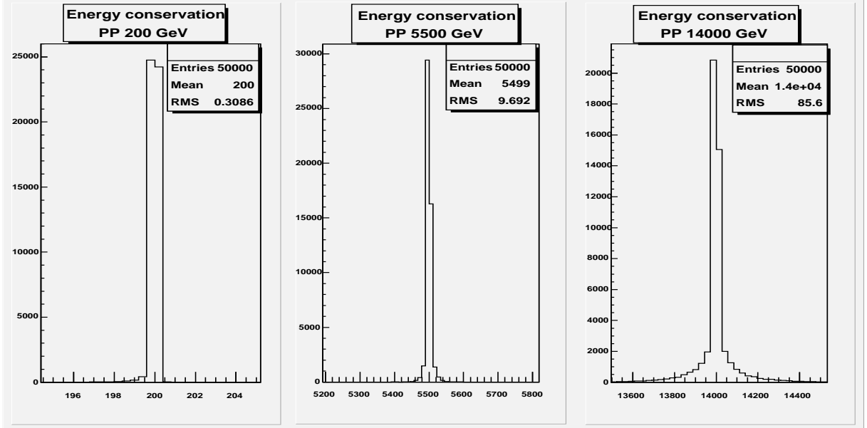
Figure 1: The energy distribution in the HIJING events
