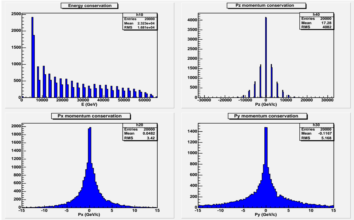
Figure 5: Properties of CC-interactions at \sqrt{s_{NN}} = 5500 GeV in the HIJING model.
