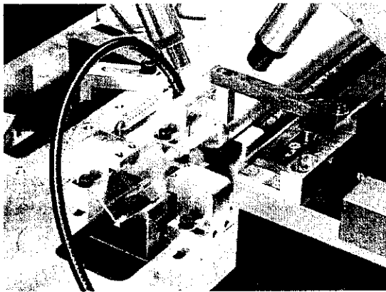
Fig. 3. Precise wire positioning using glue curing under UV illumination.
