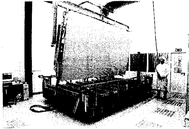
Fig. 2. The MDT prototype chamber during assembly.
