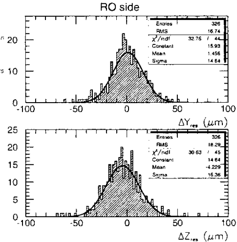
Fig. 6. Residuals of measured wire coordinates w.r.t. the expected grid.
