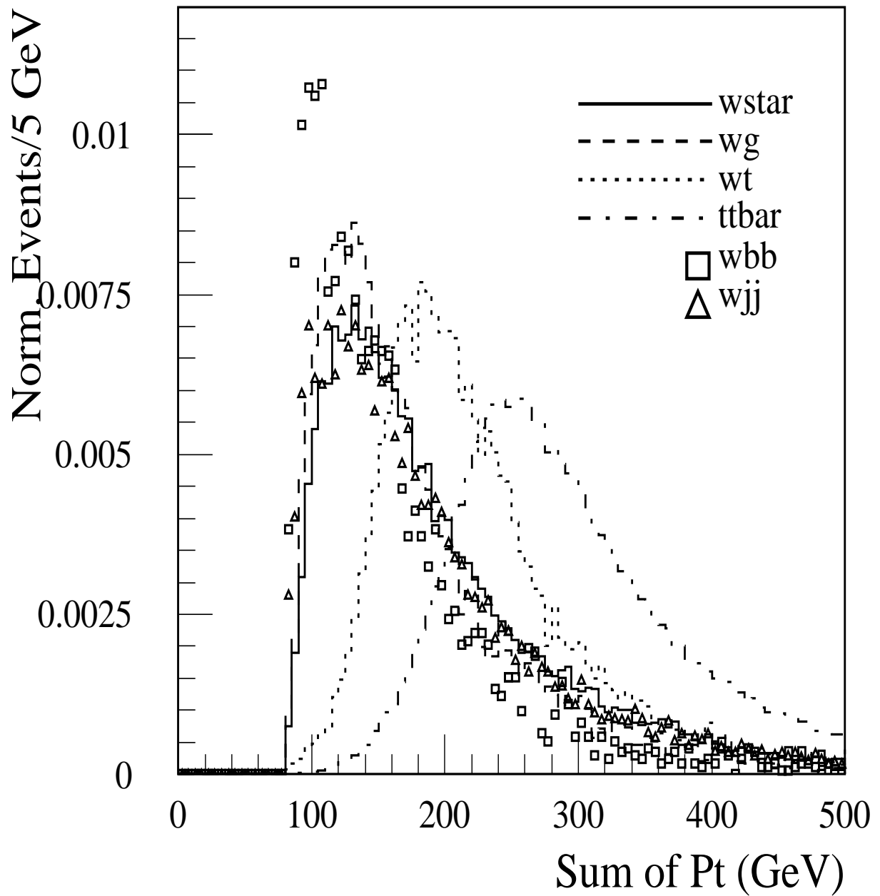
Figure 5: Scalar sum of jet P_T in each event for signal and background after ATLFASST and ATLFASST-B. Refer to text for description of event pre-selection.
