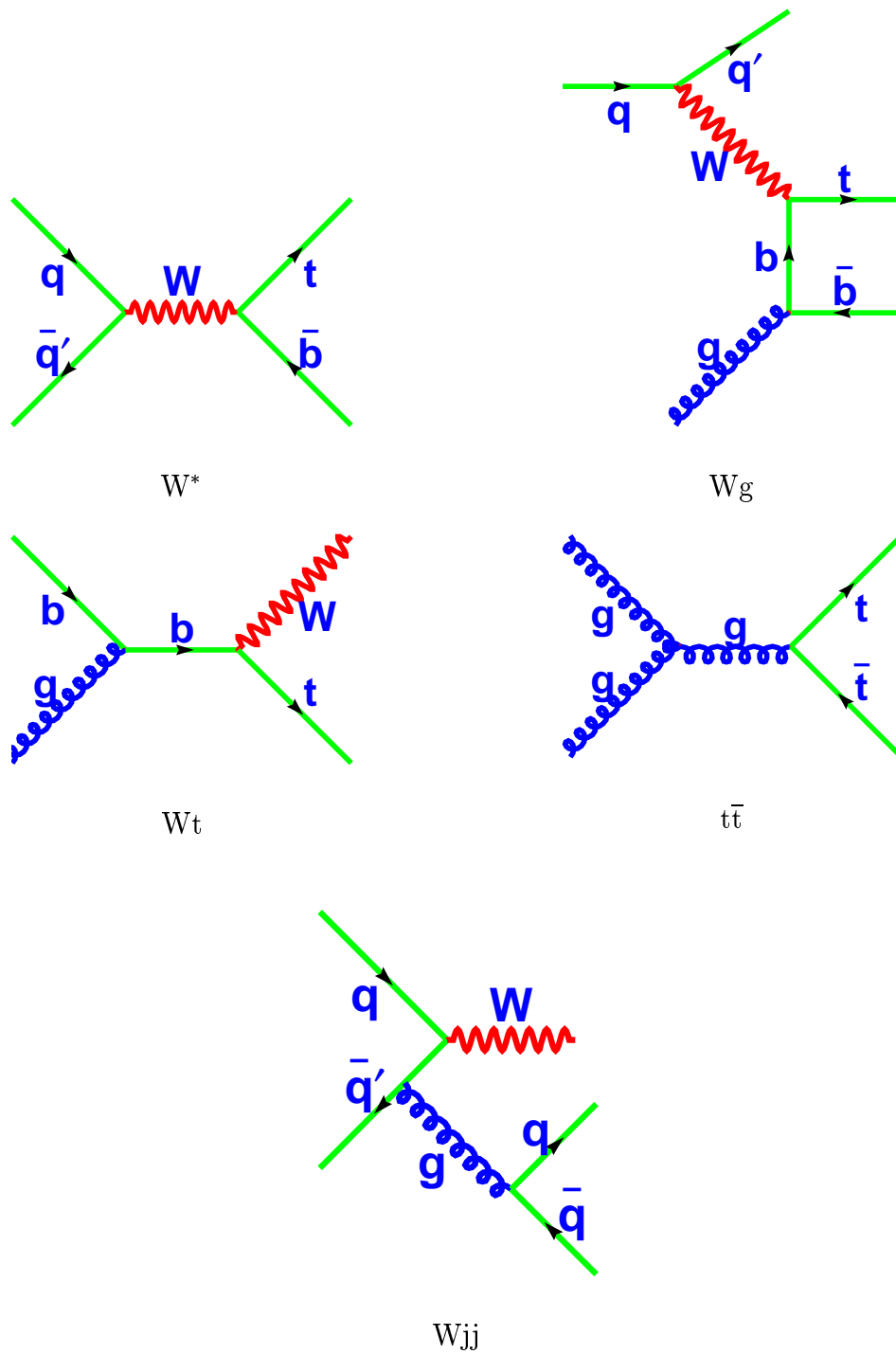
Figure 1: Single top signals and background at the LHC. Reading from left to right, top to bottom the diagrams are W^* , Wg fusion, Wt , and backgrounds t\bar{t} and Wjj .
