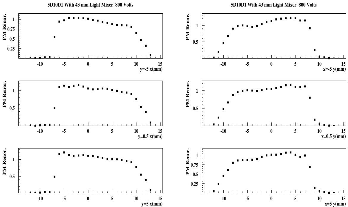
Figure 35 : Variation of the PMT (#5D10D1) response, as a function of x and y coordinate of a 1 \times 1 \text{ mm}^2 illuminated window of this PMT photocathode moving in front of the output face of the light mixer (the PMT is simply used as a spot photodetector). The signal of that spot photodetector, after pedestal subtraction is renormalised to the averaged response on a 16 \times 16 \text{ mm}^2 central square window on the output face of the "light mixer". The length of the "light mixer" was 43 mm, and the fiber points to the top left corner on the "light mixer" input face.
