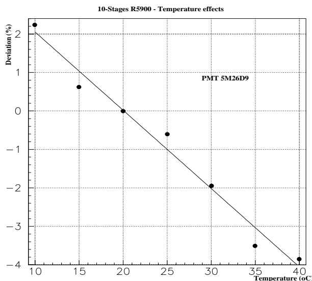
Figure 46 : Temperature effect on the amplification of a typical R5900. The gain variation is of the order 0.2% per 1^\circ \text{C} .
