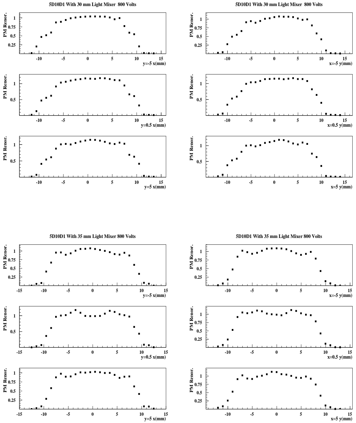
Figure 34-a : Variation of the PMT (#5D10D1) response as a function of x ( y ) coordinate, and for different fixed values of the other coordinate. The signal after pedestal subtraction is renormalised to the averaged response on a 16 \times 16 \text{ mm}^2 central square window on the output face of the light mixer. The length of the "light mixer" was 30 mm (top) and 35 mm (bottom).
