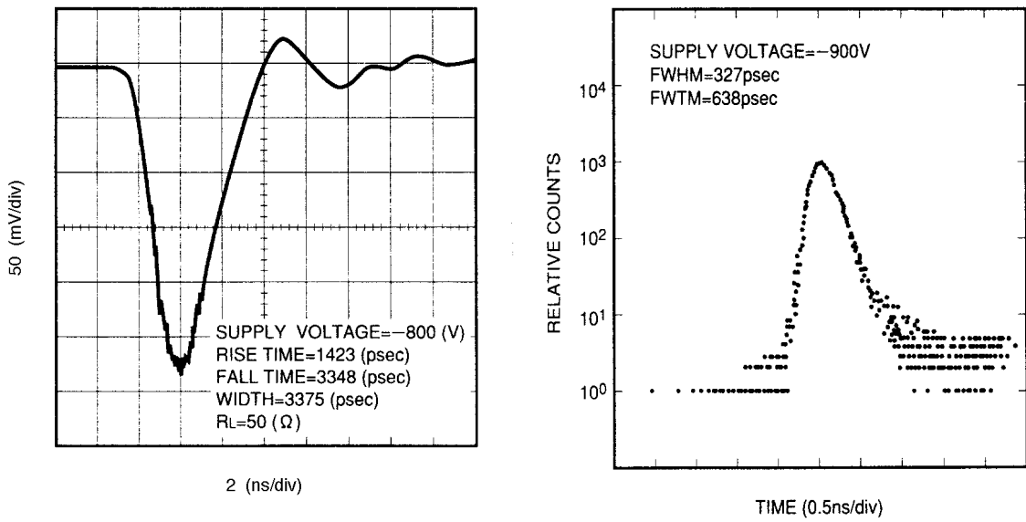
Figure 7: Typical temporal response of the R5900 series: typical time response on the left. Typical Transit Time Spread on the right (Hamamatsu documentation).
