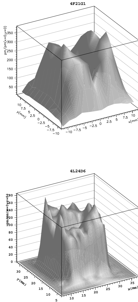
Figure 27 : Surface representation of the variation of the response of two R5900: #4F21G1 of the first generation and #4L24D6 of the second generation. For the 4F21G1, the light spot was achieved using a large aperture emission cone so that the scanning resolution was 2 mm. For the 4L24D6, the scanning resolution was decreased to 1 mm using a fiber with a smaller light aperture emission cone.
