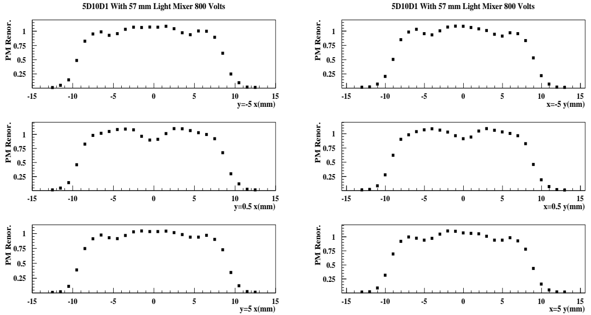
Figure 34-c : Same as on Figure (34-a). The length of the "light mixer" was 57 mm.
