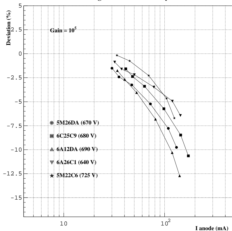
Figure 66 : Linearity deviation of a set of 5 PMTs, used in Module 0, measured at the nominal amplification, with the 2.5:2.5:1:1-1:2.5:2.5 voltage repartition. For these measurements, the experimental set-up is the one presented on Figure (44): the variation of the pulsed light amplitude is achieved using a set of different attenuation neutral filters. The 2% linearity deviation corresponds to a PMT anode current range of 30 to 60 mA, and with a pulse width of 17 ns, in a photoelectron range of 32K to 64K. 50 K photoelectron with an amplification of 10^5 corresponds to a resulting PMT anode current equal to 50 mA
