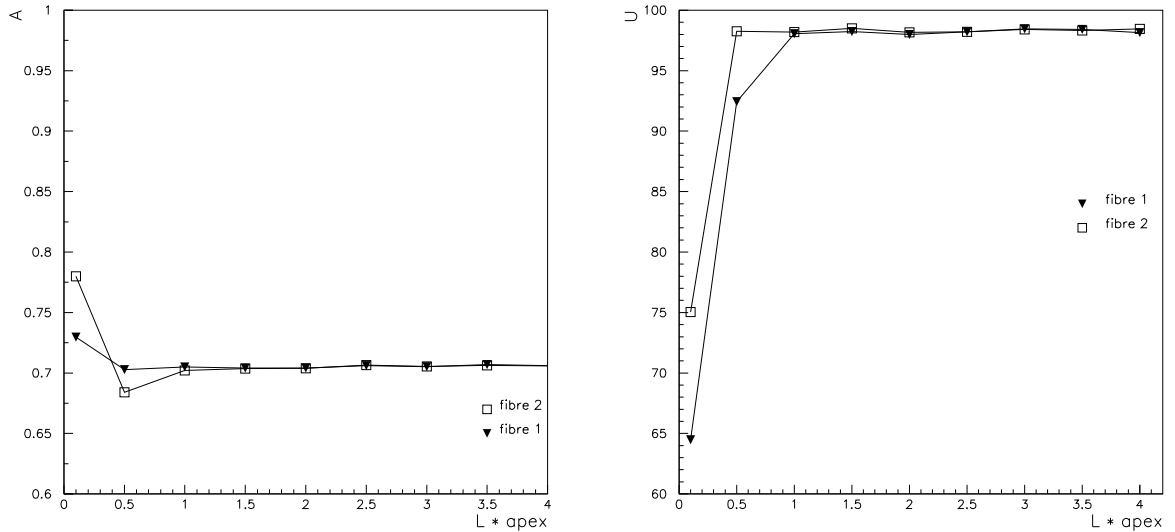
Figure 31 : Monte Carlo results on the acceptance and uniformity of PMT response as a function of the mixer length. Left part of the figure shows the ratio ( A ) of photocathode light to incident light. Right part of the figure shows the uniformity ( U ) of illumination of the photocathode. The results are shown for fibres near (#1) or far (#2) from the center of the light mixer.
