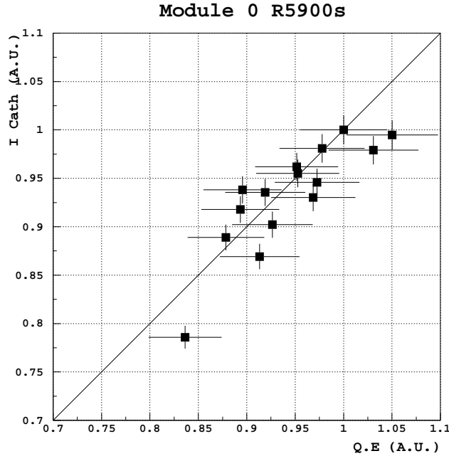
Figure 24 : Correlation between the estimated 480 nm quantum efficiency ( x -axis), and the photocathode current measured at the "plateau" with the 480 nm interferential filter ( y -axis). For the subset of tested PMTs, one of the PMT has been used as a reference (#5M18C3). We fix to 5% the systematic error on the relative estimated 480 nm quantum efficiency, and to 1.5% the systematic error on the relative photocathode current.
