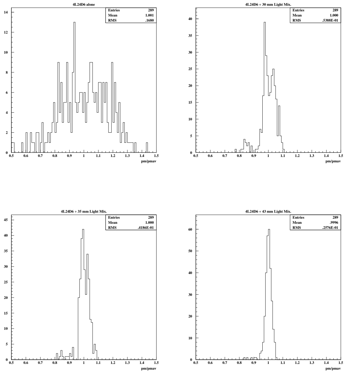
Figure 37 : Distribution of the variation of the PMT (#4L24D6) response measured in a 16 \times 16 scan of the PMT coupled without (top-left) and with a "light mixer". The length of the light mixer was 30 mm (top-right), 35 mm (bottom-left), 43 mm (bottom-right).
