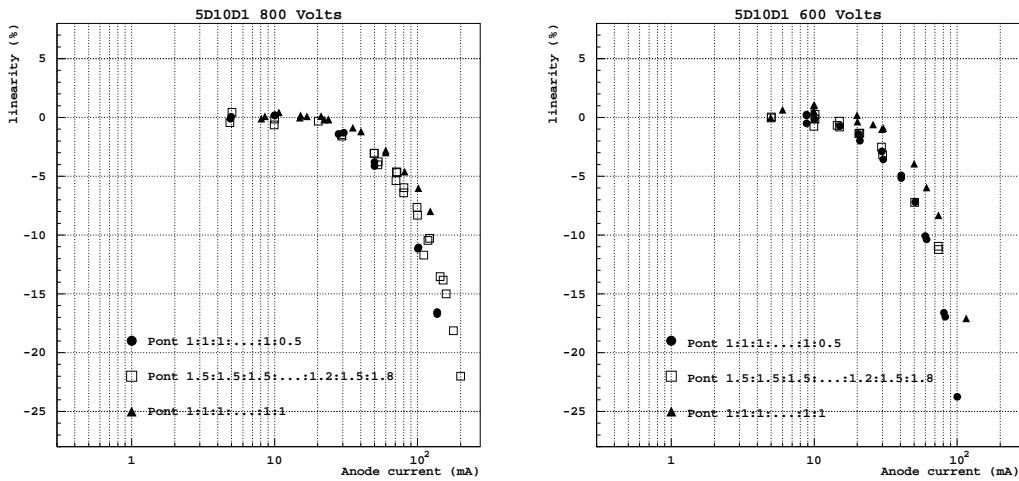
Figure 54 : R5900 linearity (PMT # 5D10D1 of the second generation), as a function of the anode current for three different voltage repartitions: open squares correspond to the 1.5:1.5:1.5:1:...:1.2:1.5:1.8 configuration, full circles to the 1:1:1:...:1:1:0.5 configuration, and full triangles to the 1:1:1:...:1:1:1 configuration. On left part, PMT voltage was set to 800 Volts, on right part to 600 Volts.
