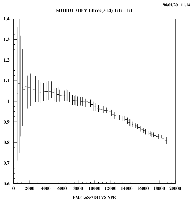
Figure 61 : Differential linearity curves with a 1:1:1:1-1:1:1 voltage repartition. Top figures correspond to a PMT amplification of 10^5 with two different ranges in N_{p.e.} . Bottom corresponds to an amplification of 10^6 .
