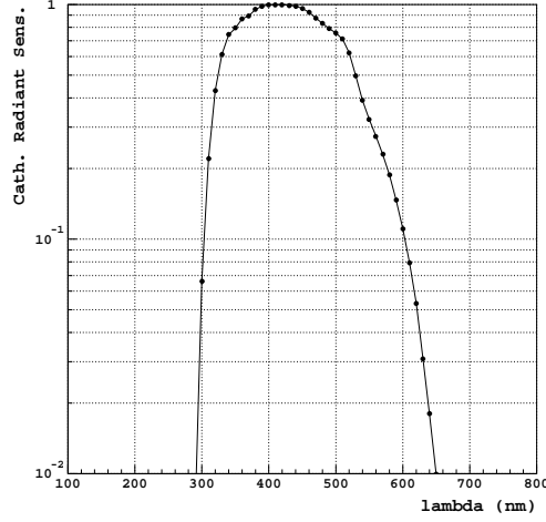
Typical R5900 Photocathode sensitivity
