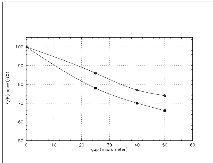
Figure 2: Girder field dependence on glue gap value. Circles - initial packing factor = 0.76, boxes - initial packing factor = 0.90.
