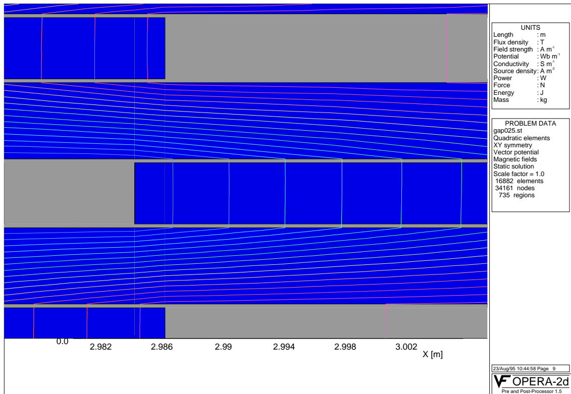
Figure 8: Flux map for 0.25 mm glue gaps.
