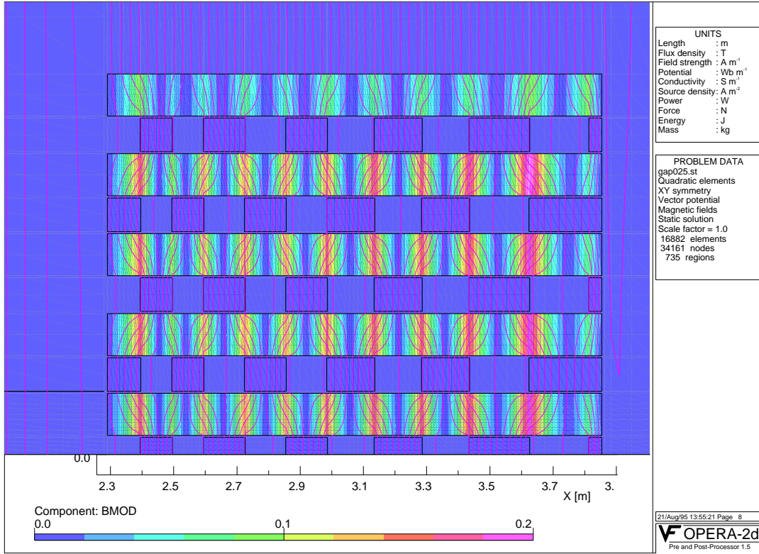
Figure 7: Flux lines waving around tiles with the 0.25 mm glue gaps in the system.
