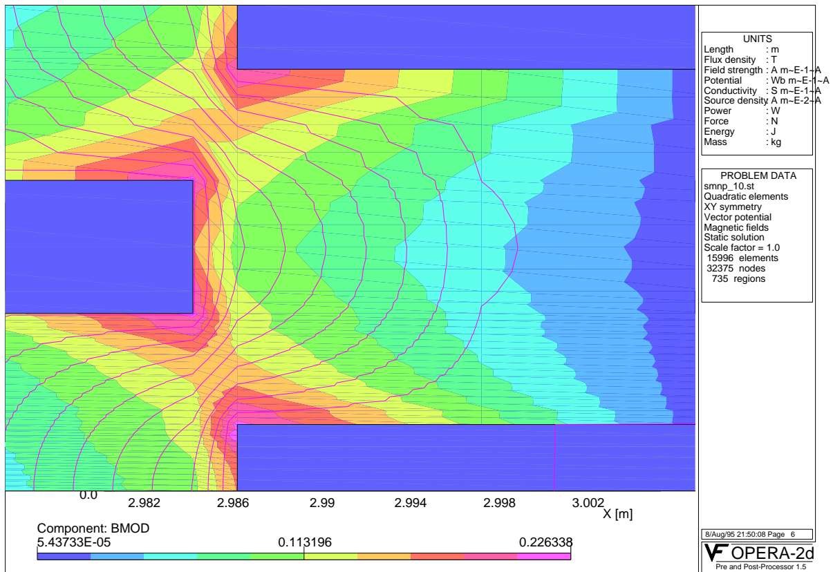
Figure 5: Flux map for no glue gaps and 2mm layers present in the system.
