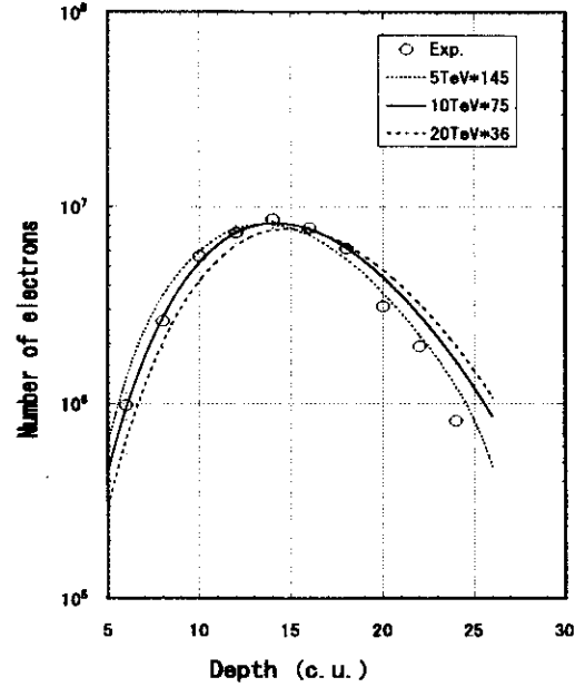
Fig. 1. Transition curve of the total electron number. The total electron number is obtained by integrating the lateral distribution of the electron density, which is obtained from the local darkness in the halo, at every sensitive layers in EC. The curves are those which are produced by N_\gamma \gamma -rays with energy \langle E \rangle , tabulated in Table 1, incident upon EC.
