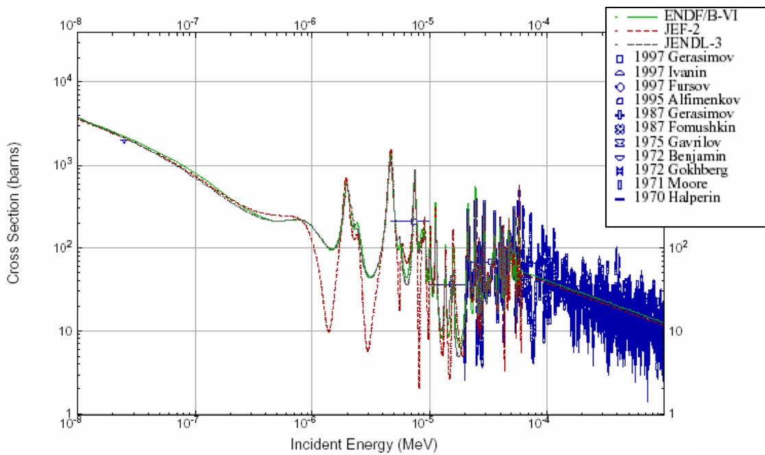
Figure A-8: fission cross section of ^{245}\text{Cm} in the low energy region.
