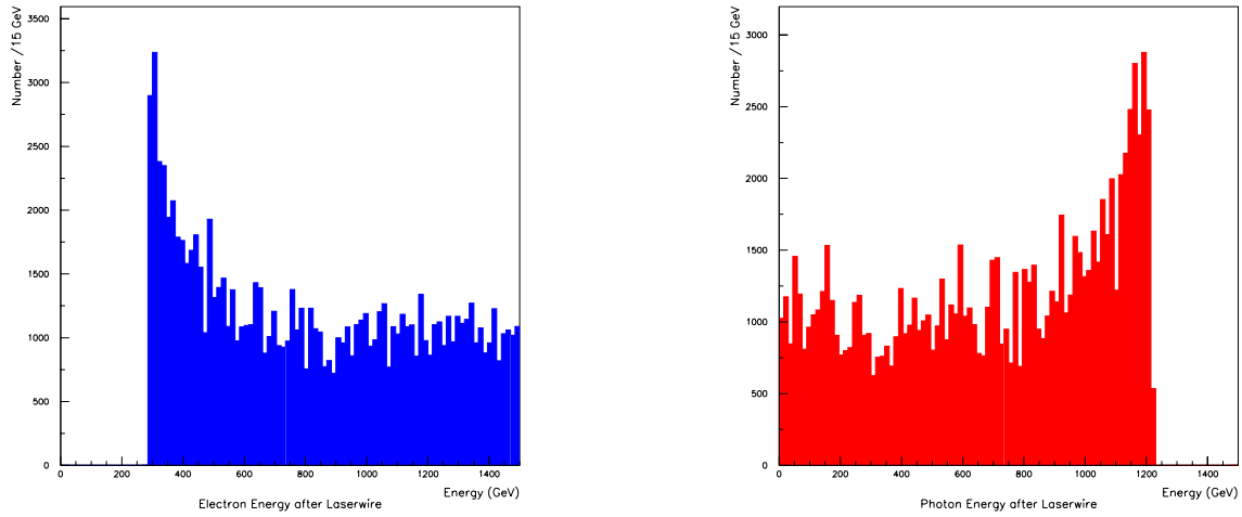
Figure 13: The energy distributions for electrons (left) and photons (right) after Compton scattering in the laserwire.
