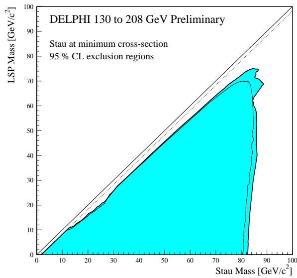
Figure 27: 95% CL exclusion region in the (M_{\tilde{\tau}}, M_{LSP}) plane obtained for the minimal \tilde{\tau}\tilde{\tau} pair-production cross-section. The shaded region shows the obtained exclusion limit, and the thin solid line shows the limit expected for no signal events.
