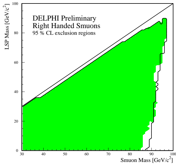
Figure 24: 95% CL exclusion region in the (M_{\tilde{\mu}_R}, M_{LSP}) plane. The shaded region shows the obtained exclusion limit, and the solid line shows the expected limit treating simulated background as data.
