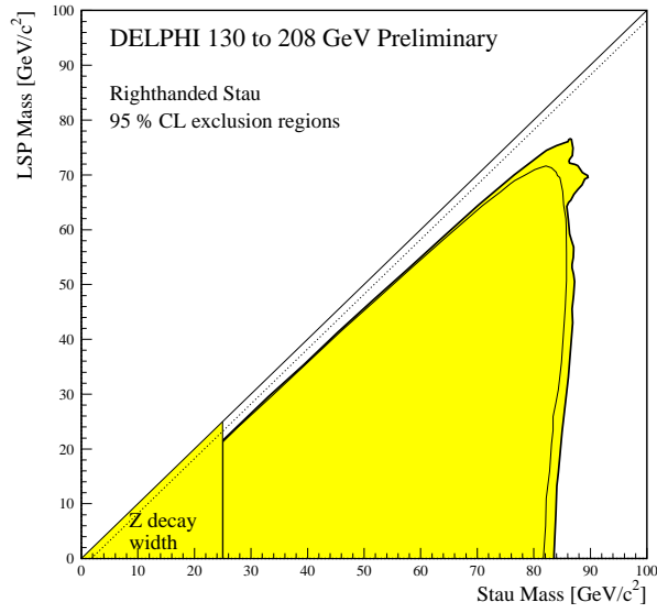
Figure 26: 95% CL exclusion region in the (M_{\tilde{\tau}_R}, M_{LSP}) plane. The shaded region shows the obtained exclusion limit, and the thin solid line shows the limit expected for no signal events.
