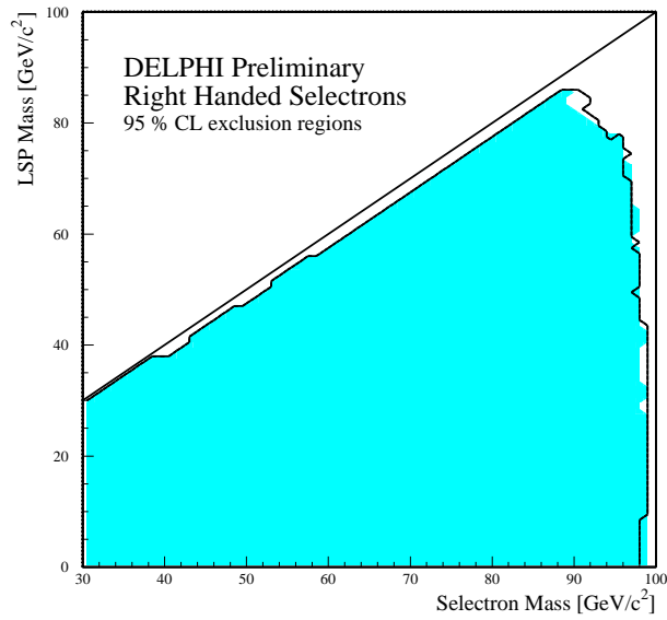
Figure 23: 95% CL exclusion region in the (M_{\tilde{e}_R}, M_{LSP}) plane. The shaded region shows the obtained exclusion limit, and the solid line shows the expected limit treating simulated background as data.
