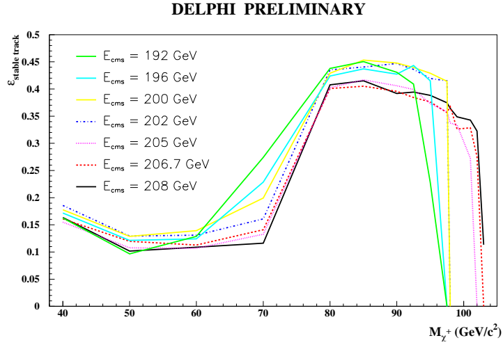
Figure 16: Efficiency for selecting a single almost stable chargino, as function of its mass, at the reference centre-of-mass energies collected by DELPHI in the years 1999 and 2000.
