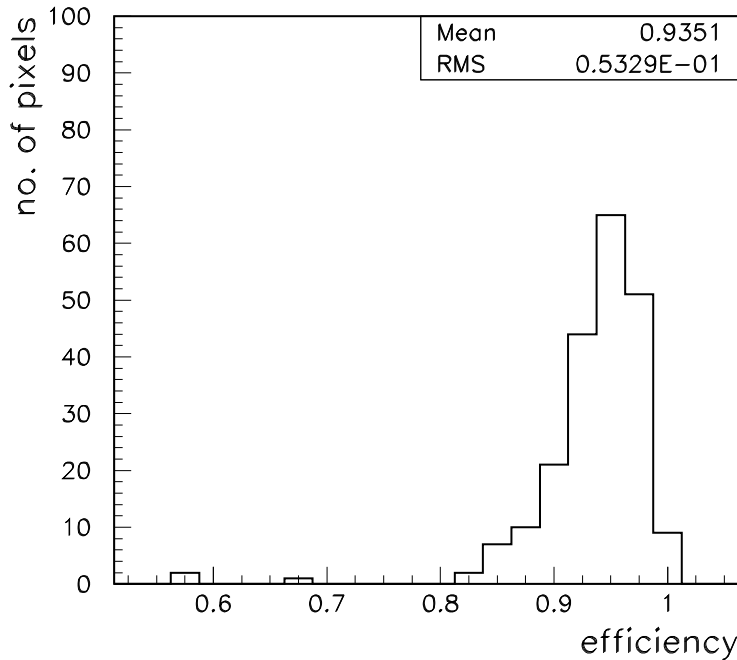
Figure 2: Efficiency distribution of a diamond pixel detector operated at 1600 e threshold.
