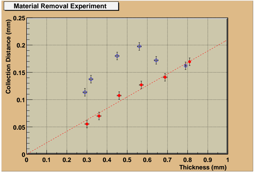
Figure 6: Thinning of two CVD diamond samples (DB91 and DB92). The charge collection distance measured as a function of the thickness after thinning on the growth side of DB91 and on the nucleation side of DB92.
