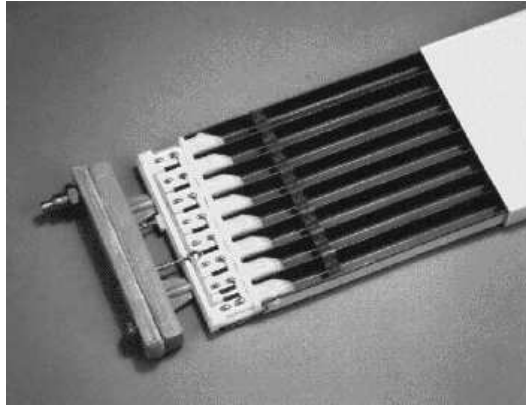
Figure 3.11: Photograph of a streamer tube.
