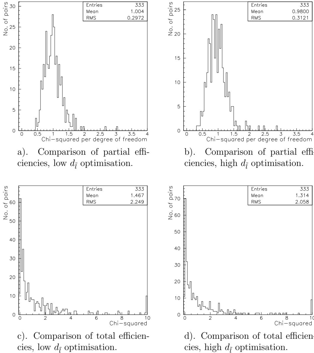
Figure 7.5: The \chi^2 distributions resulting from compatibility tests between 189 and 208 GeV Monte Carlo data. In the two lower plots not all pairs of points gave a \chi^2 in the range shown. Such pairs have been placed in the last bin. Good agreement is shown amongst all the partial efficiencies, and most of the total efficiencies.
