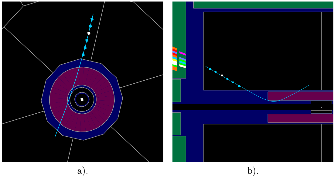
Figure 5.7: An example of a track with \mathcal{R}_{\tilde{\tau}} = 1 from signal Monte Carlo, viewed in (a) the r\phi plane and (b) the \rho z plane ( \rho is equal in magnitude to r , but with a sign that makes it negative for a certain half of the \phi range which is chosen to make the event as clear as possible). Although the d_0 of the track shows that the slepton reached a radius above at least one VDET layer before decaying, it did so at such a high |\cos(\theta)| that it did not produce hits.
